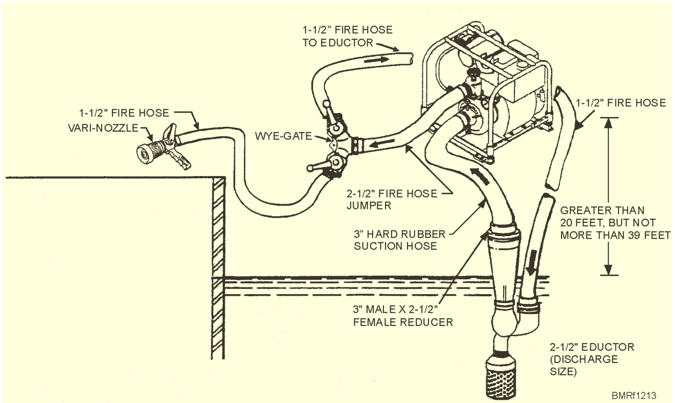
Figure 12-13.—Firefighting hookup.
