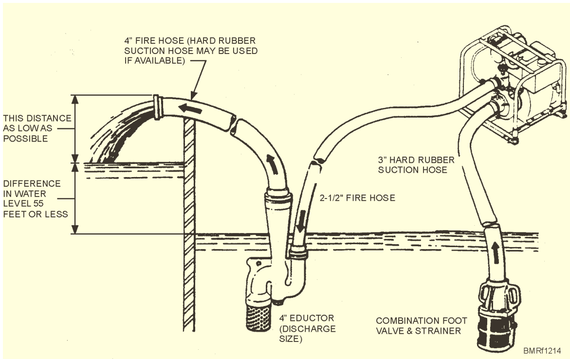
Figure 12-14.—Dewatering hookup.
