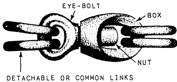
Figure 4-7.—Mooring swivel.
