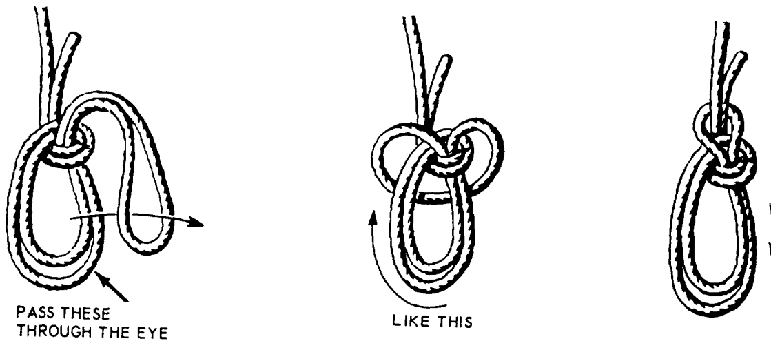
Figure 3-16.—Bowline on a bight.
