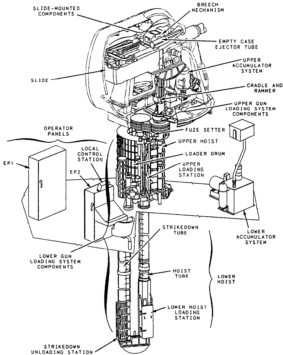
Figure 6-17.—The 5"/54 Mk 45 gun loading system, major components.
