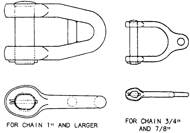
Figure 4-6.—Mooring shackles.
