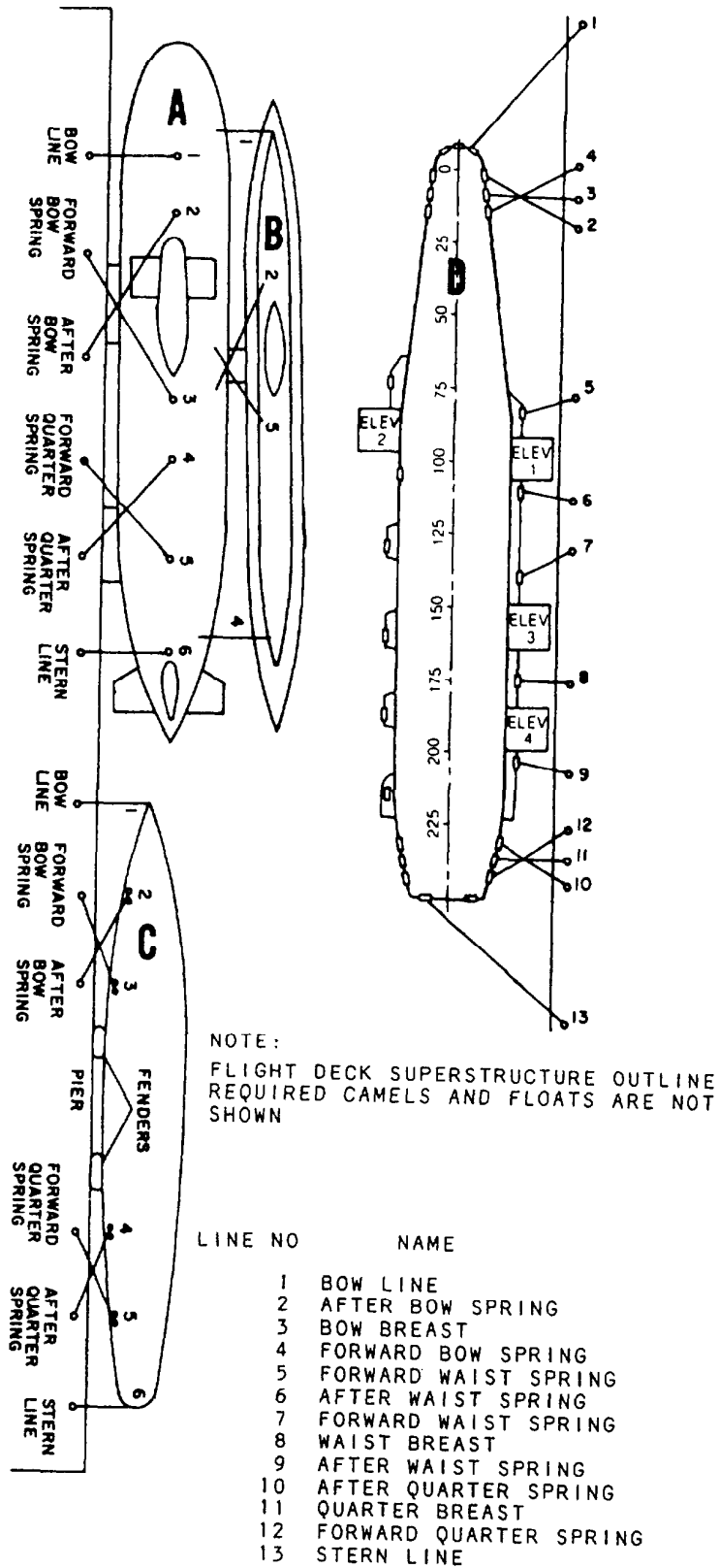
Figure 4-35.-Mooring lines.
