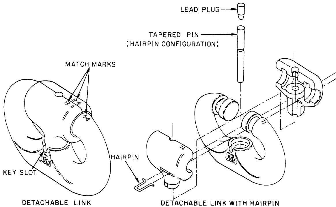
Figure 4-2.—Detachable link.
