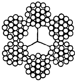
6 STRANDS OF 19 WIRES (6X19)
