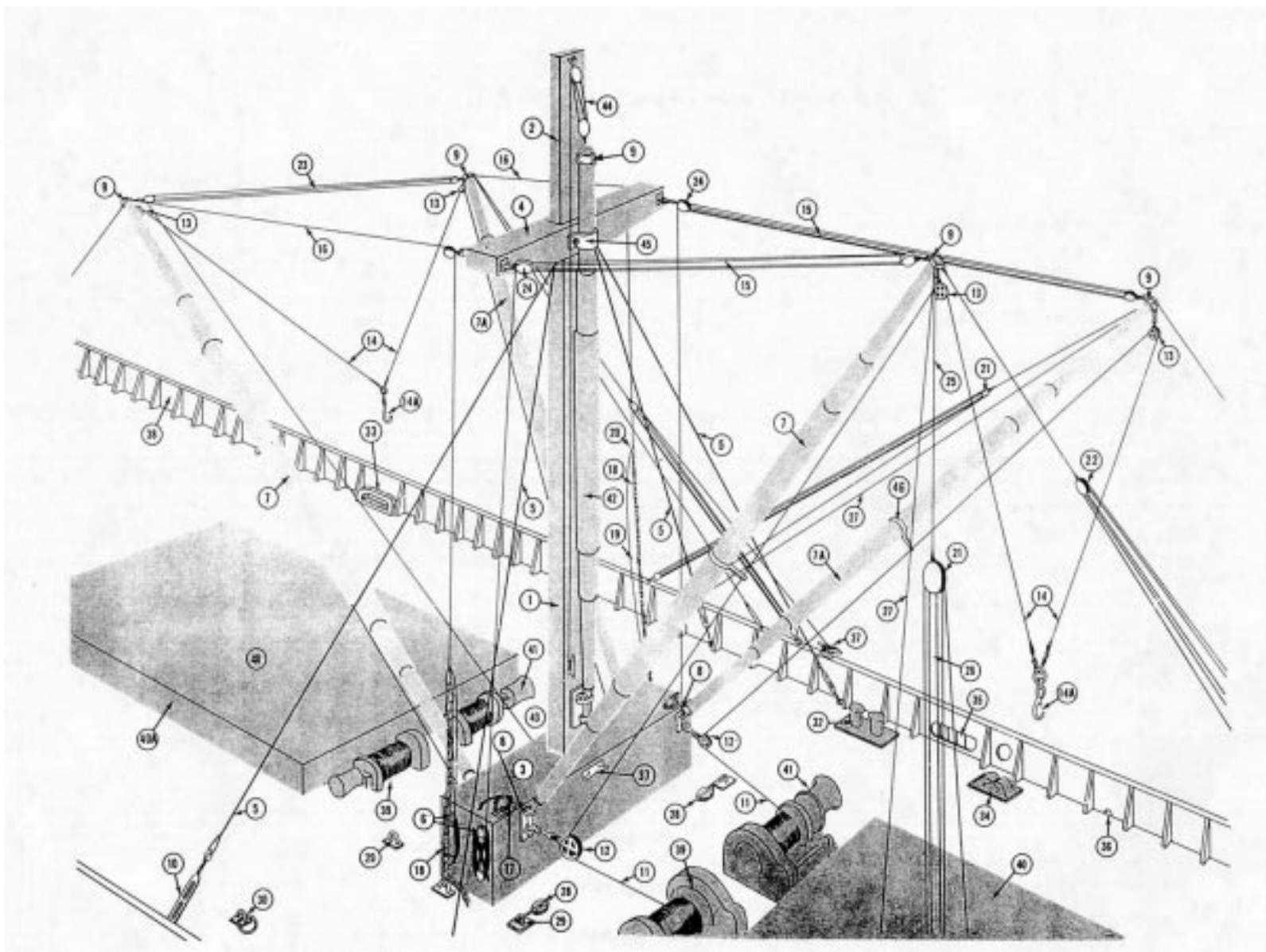
Figure 4-21.-Yard-and-stay rig.
