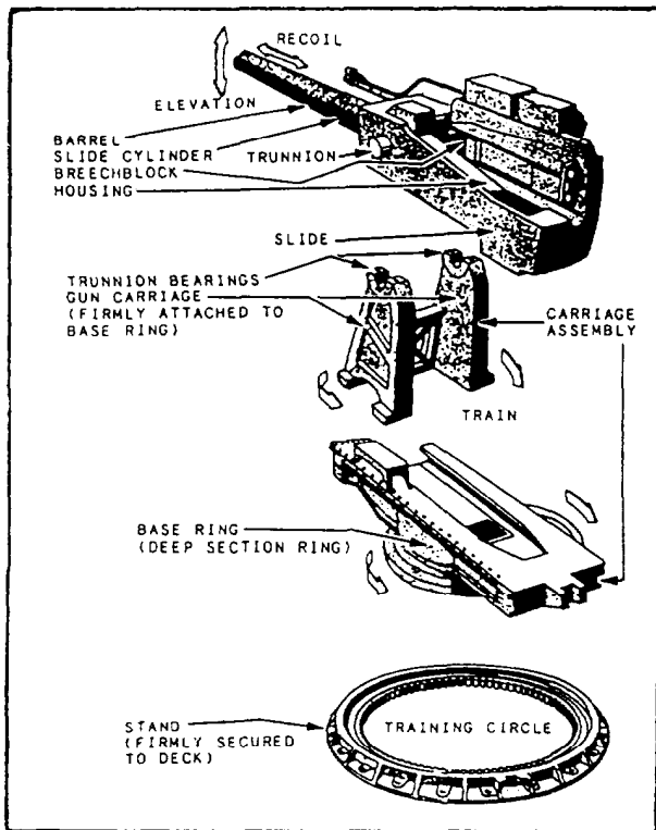
Figure 6-10.—Gun-positioning equipment.
