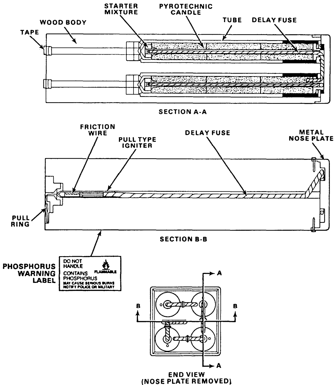
Figure 6-7.—The Mk 6 Mod 3 marine location marker.
