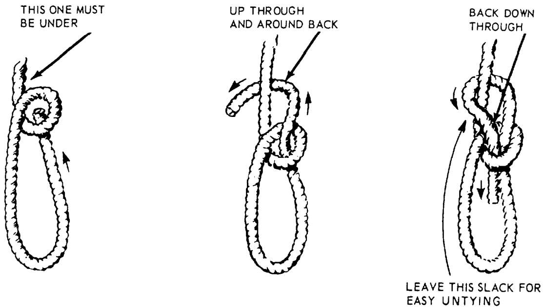
Figure 3-15.—Tying a bowline.
