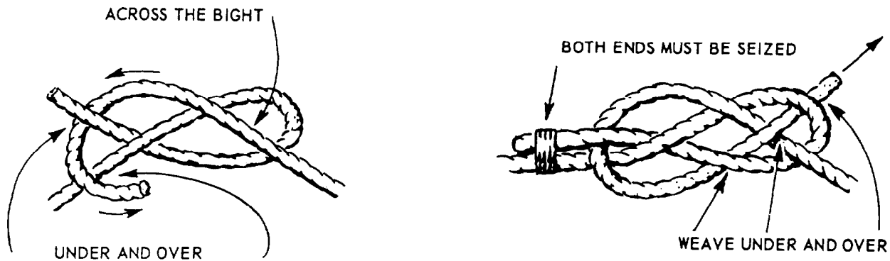
Figure 3-14.—Tying a carrick bend.
