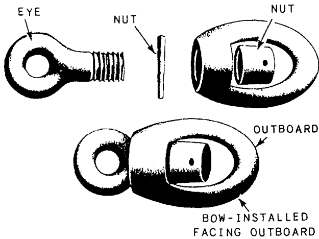
Figure 4-3.—Chain swivel.
