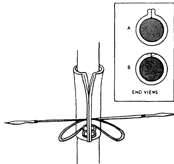
Figure 3-40.—Shoemaker's stitch.
