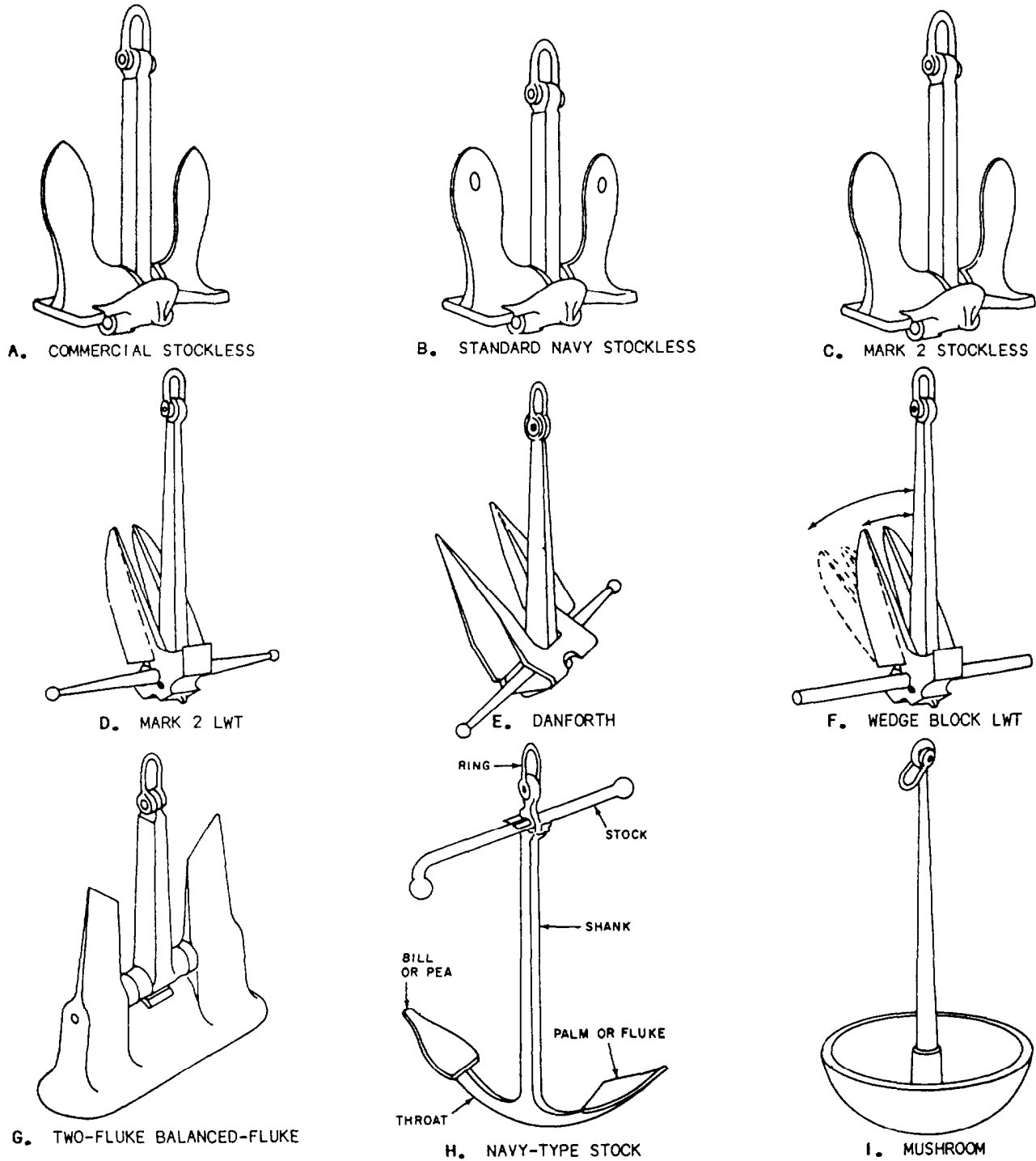
Figure 4-1.—Types of anchors.
