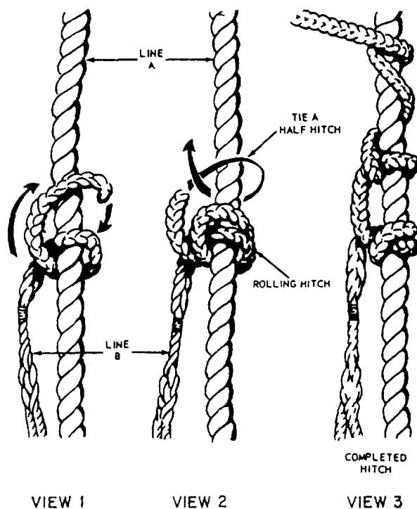
Figure 3-18.—Rolling hitch.
