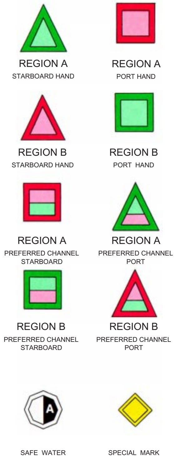
Figure 5-33.-IALA Maritime Buoyage System lateral daymarks. C69.226
