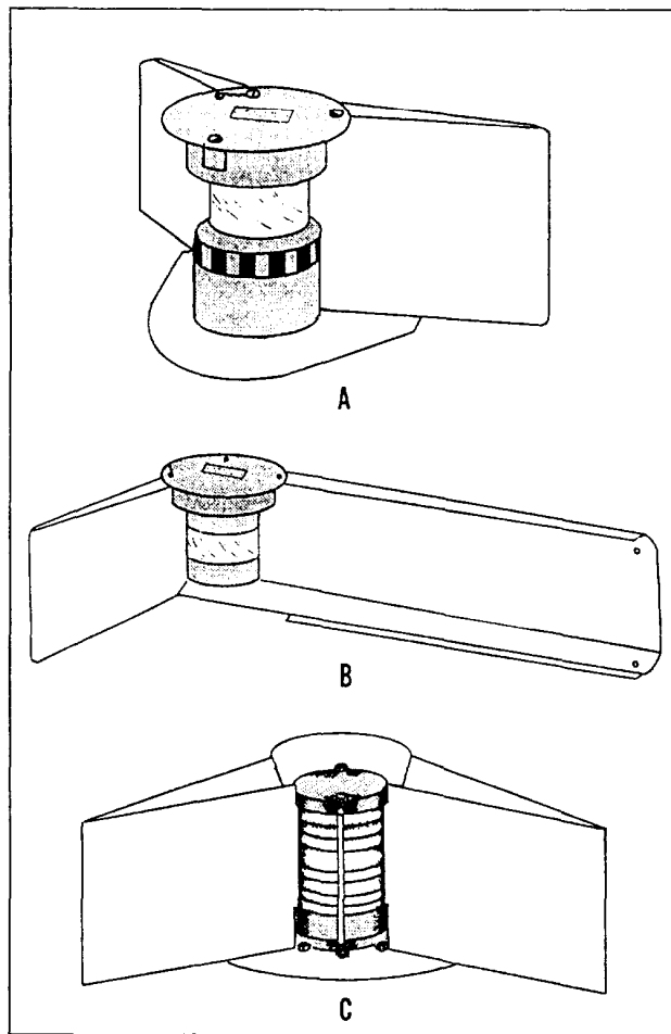
Figure 2-16.— Running lights.
