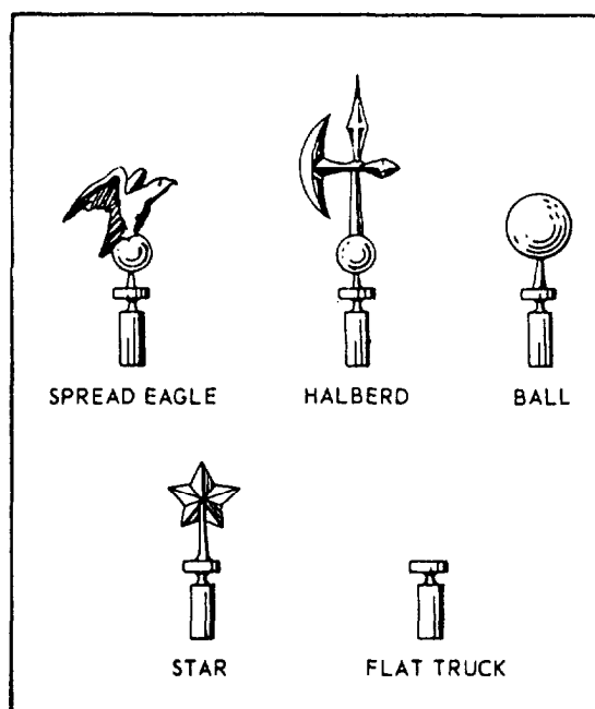
Figure 5-11.—Flagstaff insignia.
