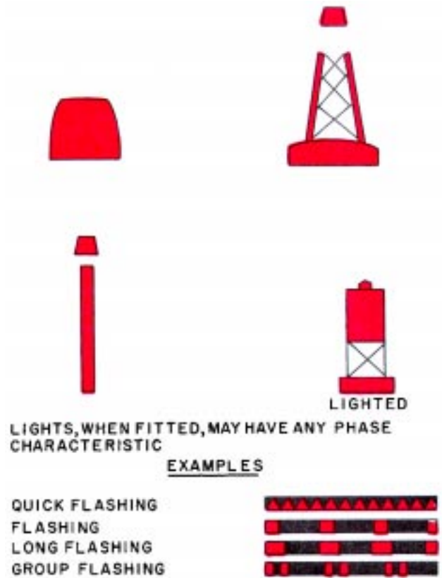
Figure 5-21.—IALA Maritime Buoyage System, International Buoyage Region A port-hand marks (buoys). C69.214
