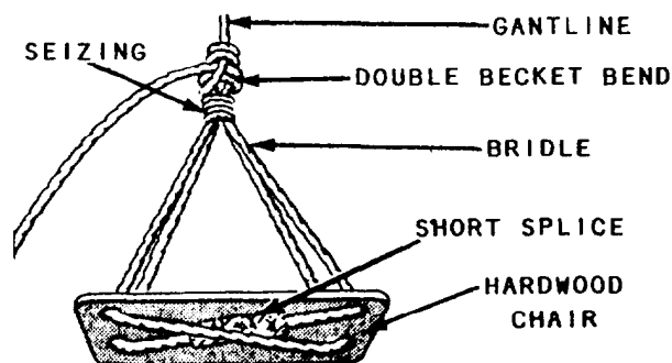
Figure 4-29.— The boatswain's chair.
