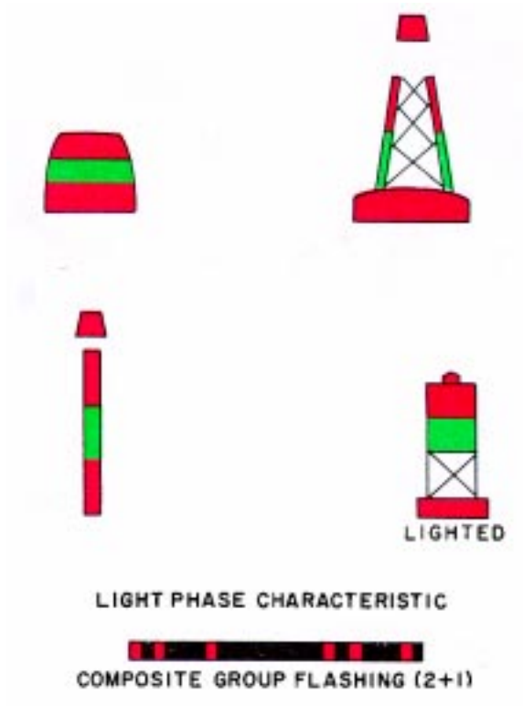
Figure 5-24.—IALA Maritime Buoyage System, International Buoyage Region A preferred channel to starboard.
