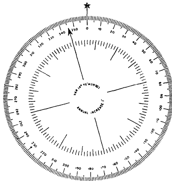
Figure 2-4— Compass rose.
