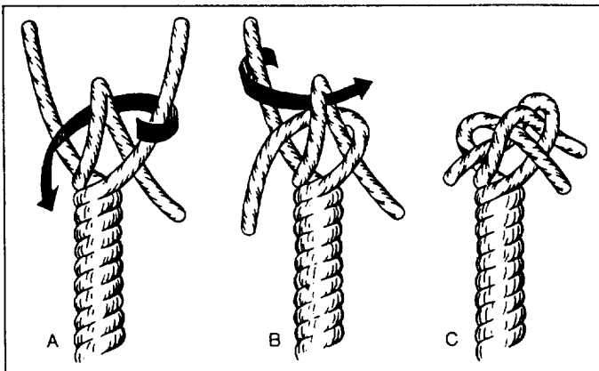
Figure 3-8.—Steps in making a crown.
