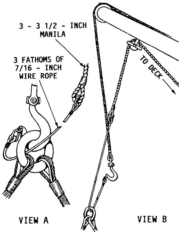
Figure 5-8.—Safety runner.
