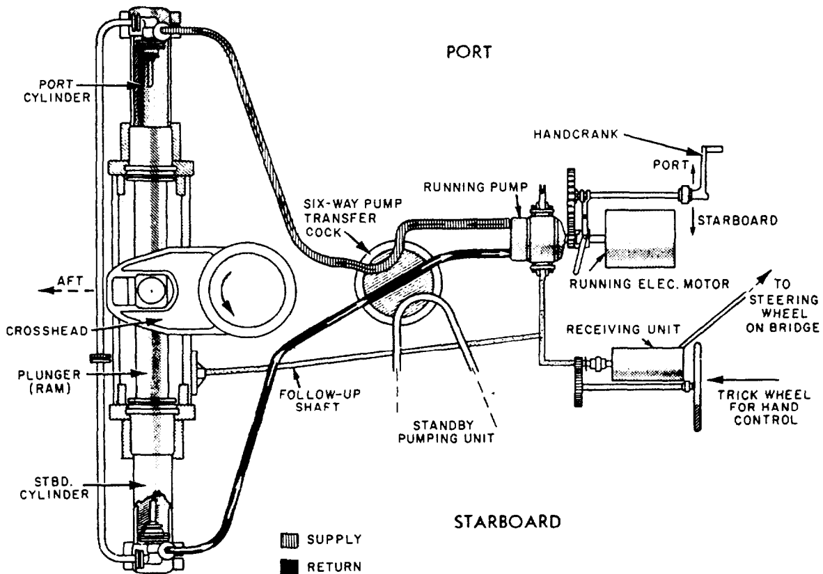
Figure 2-6— Single-ram electrohydraulic steering gear system.
