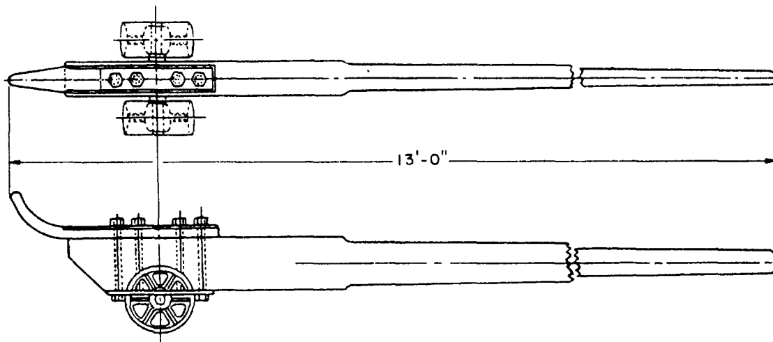
Figure 4-8.—Cable jack.
