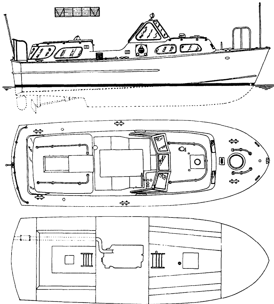
Figure 5-3.-33-foot personnel boat.
